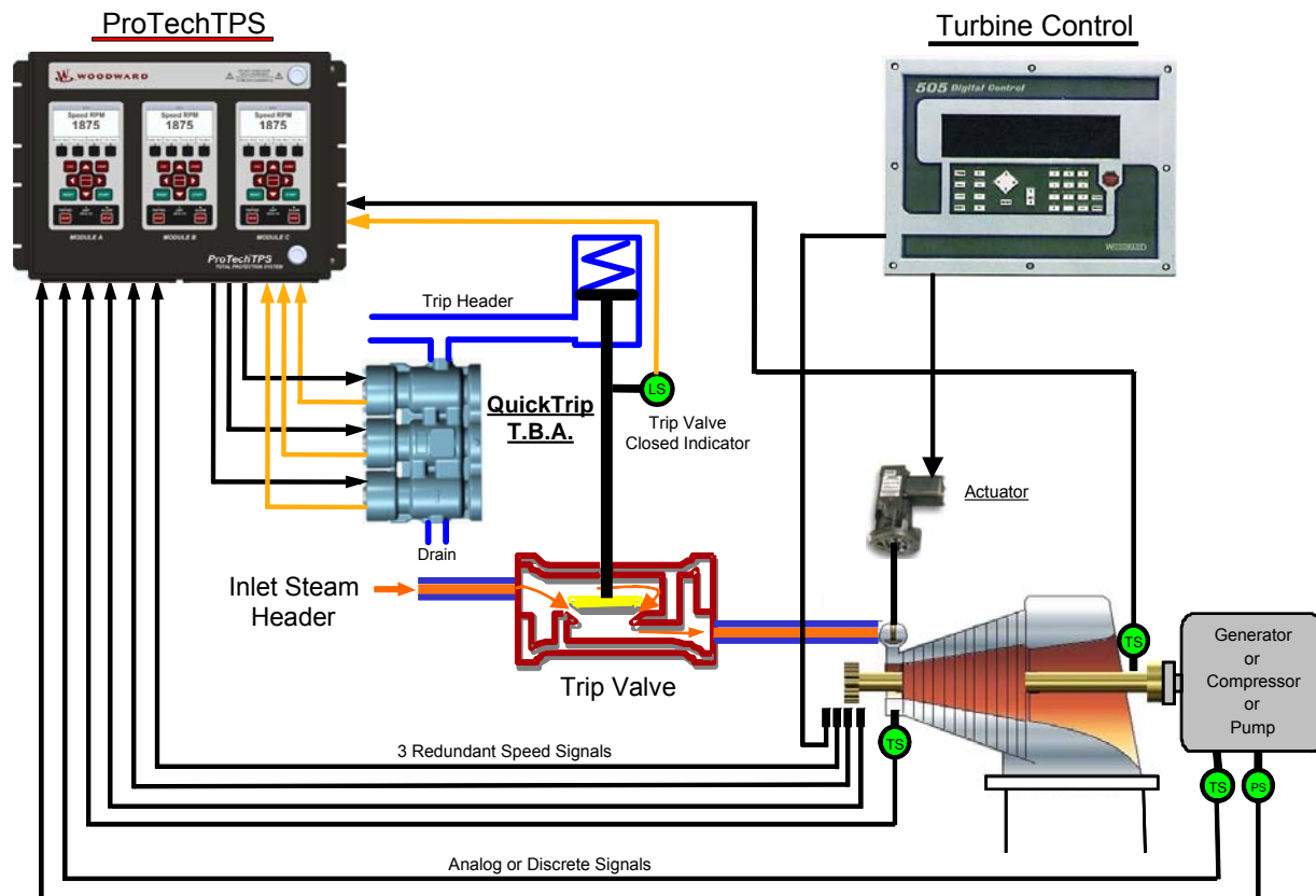
Figure 1. Typical QuickTrip Application
