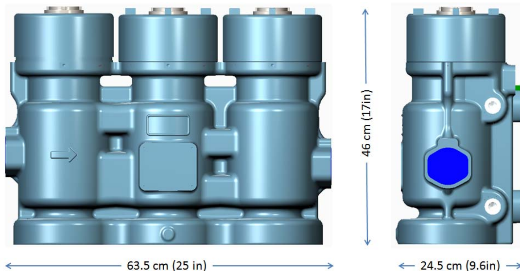
Figure 2. QuickTrip Outline Dimensions
